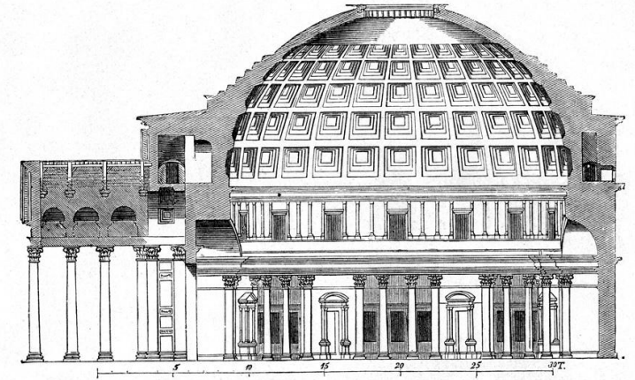
13. The Pantheon at Rome. Section. Built 26 B. C., restored 202 A. C.
